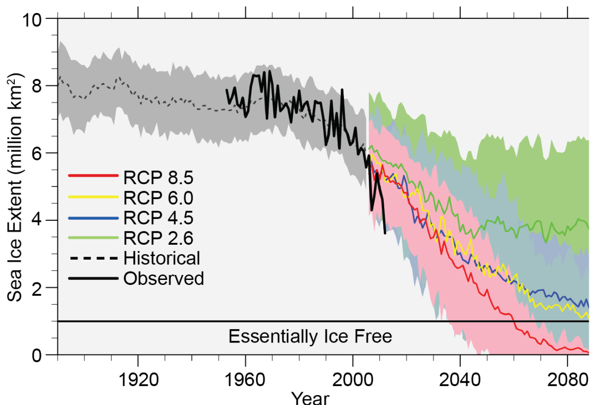
Figure 2: Observed and model projections of Arctic sea ice melting under various assumptions about future greenhouse gas emissions. Of the modeled scenarios, emissions corresponding to RCP 2.6 would be the lowest and those corresponding to RCP 8.5 the highest. (Source: National Climate Assessment 2014, Figure 2.29 (p. 48). Adapted from Stroeve et al. 2012)
