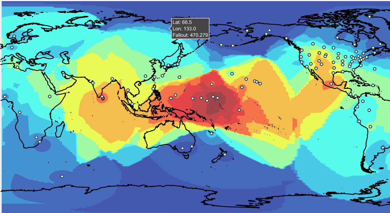
Castle Series Cumulative Fallout (log scale)
